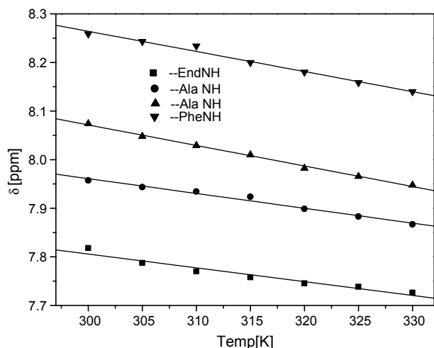
Figure 2. Temperature dependence of NH chemical shifts of peptide 1.
