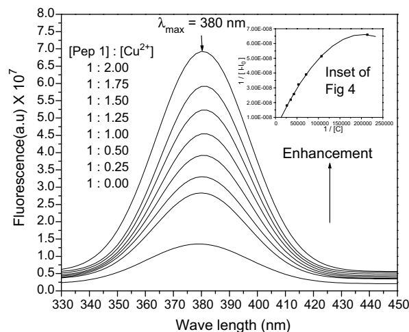
Figure 4. Fluorescence emission spectra of \text{Cu(II)} titration of peptide 1. Excitation wavelength was 320 nm. Initial conc of 1 was 1.87 \times 10^{-5} M in TFE.
