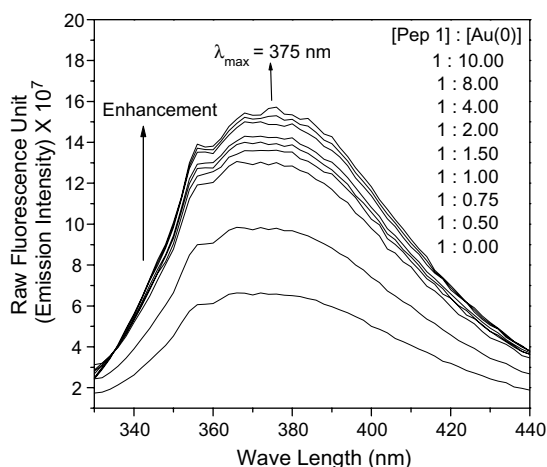
Figure 5. Fluorescence emission spectra of Au(0) titration of peptide 1 . Excitation wavelength was 320 nm. Initial concd of Au(0) was 10^{-3} M in THF.
