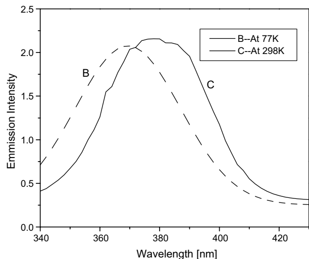
Figure 3. Fluorescence at 77 and 298 K.
