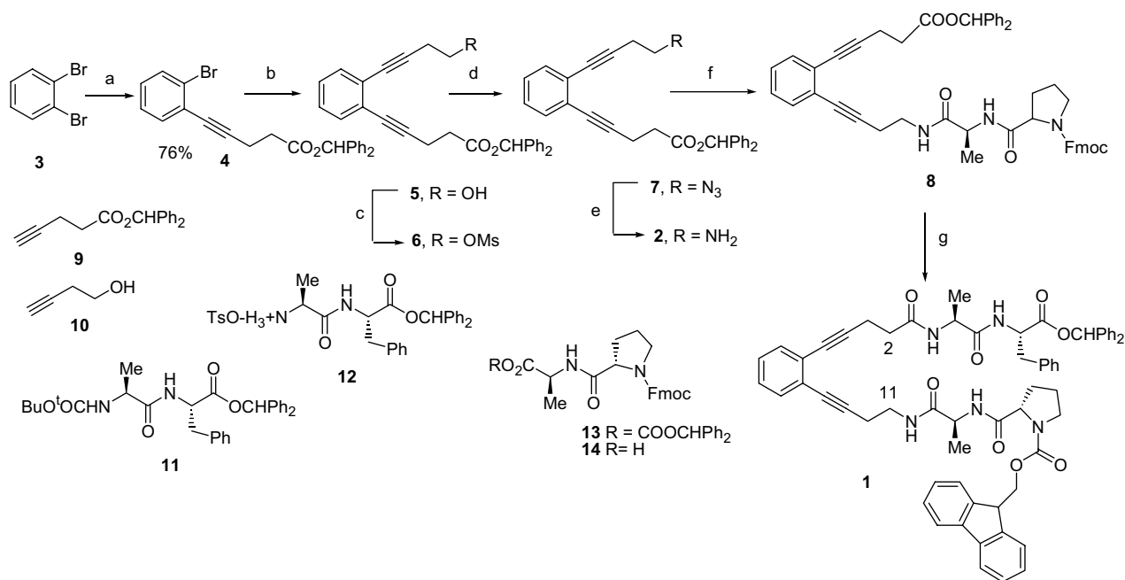
Scheme 1. Reagents and conditions: (a/b) \text{Pd}(\text{PPh}_3)_4 , \text{Et}_3\text{N} , 9/10 , \text{Cu}_2\text{Br}_2 ; (c) \text{MsCl} , \text{CH}_2\text{Cl}_2 ; (d) \text{NaN}_3 , DMF; (e) \text{PPh}_3 , \text{THF-H}_2\text{O} ; (f) 14 , EDC, HOBT; (g) (i) TFA/anisole/ \text{CH}_2\text{Cl}_2 , (ii) 12 , EDC, HOBT, \text{CH}_2\text{Cl}_2 -DMF.
