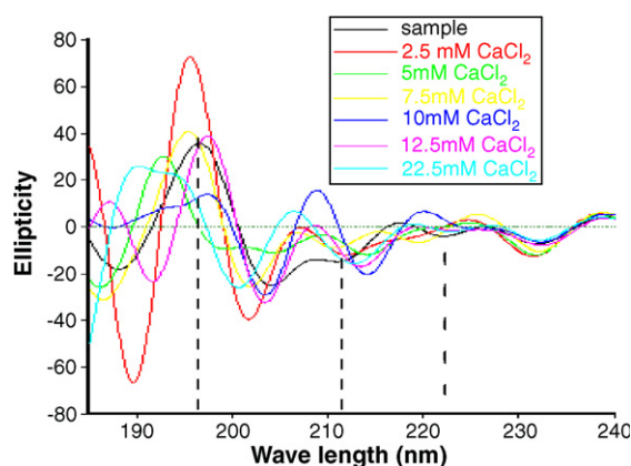
Figure 1. Overlaid deconvoluted CD spectra of peptide 1 (333 mM) in MeOH in the absence and presence of various amounts of \text{CaCl}_2 .
