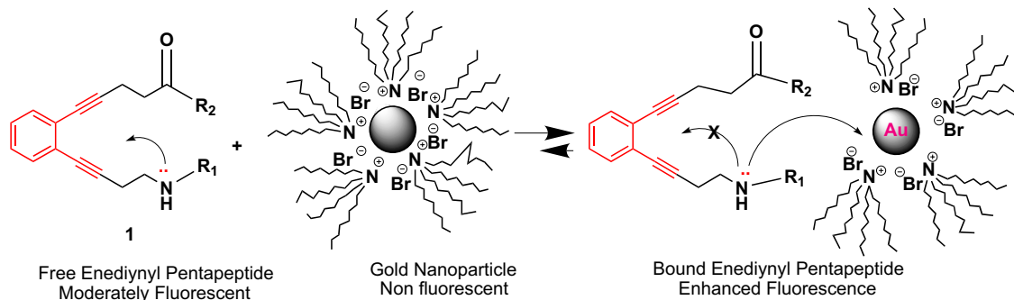
Figure 6. Probable mode of fluorescence enhancement by gold nanoparticle.
